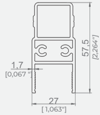
22MM CAM PANEL YAN PROFİL 22MM GLASS PANEL SIDE PROFILE
