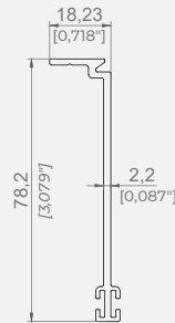
YAN RAY ORTA PROFİL SIDE RAIL MIDDLE PROFILE
